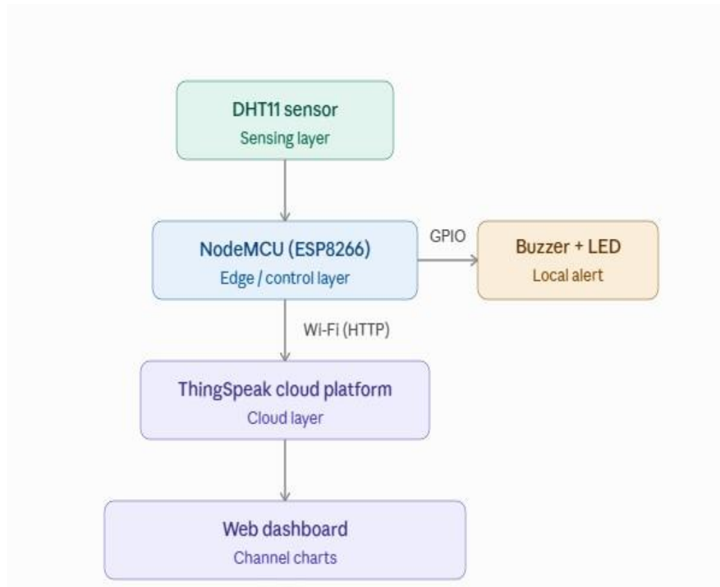
Fig. 1 Layered IoT system architecture
