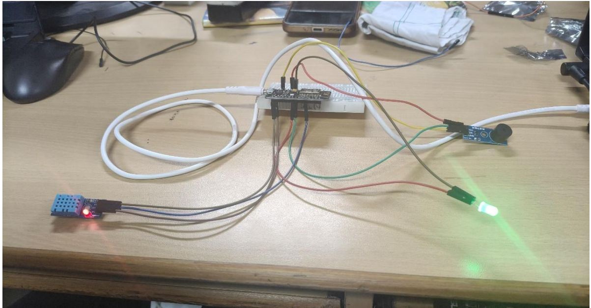
Fig. 3 Assembled prototype — DHT11, buzzer, LED wired to NodeMCU
